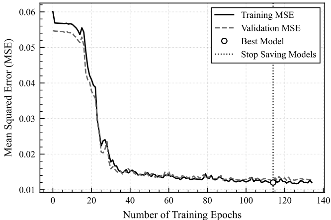
Learning Curve of MHSA-LSTM Model for SolarPlant-1 (Gyeongju)
